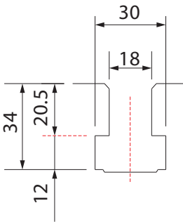
T-slot Dimensions
