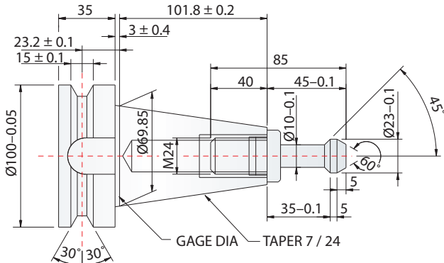
BT50
